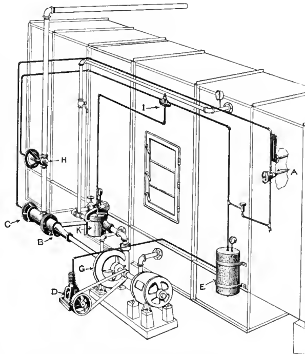
FIG. 10. DETAILS FOR THE AUTOMATIC CONTROL OF HUMIDITY BY MEANS OF AN AIR WASHER
